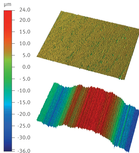
Comparison EXAKT Band saw (upper image) with wire saw (below)
